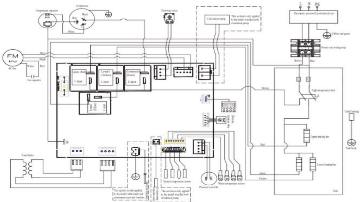
Figure 16 Electrical wiring diagram
